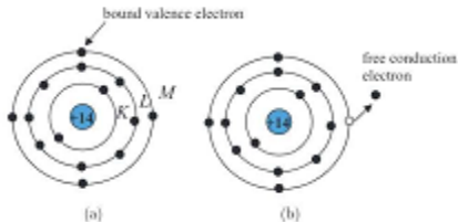
Fig. 1.1 (a) Schematic depiction of an atom using silicon with 4 electrons in the outermost shell M as an example, (b) valence electron acquires energy sufficient to overcome binding energy and to become a free conduction electron.
