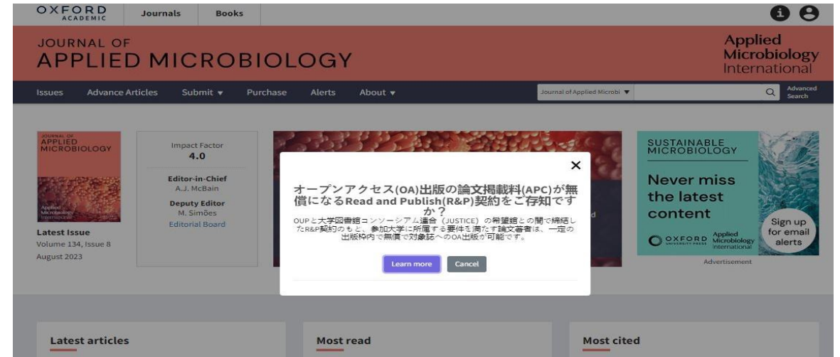
Example: JUSTICE
